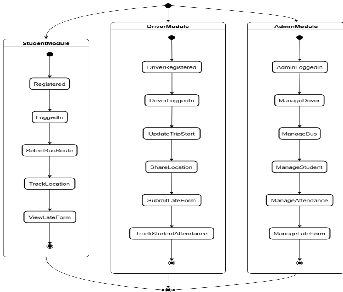
Fig.5.State Diagram
