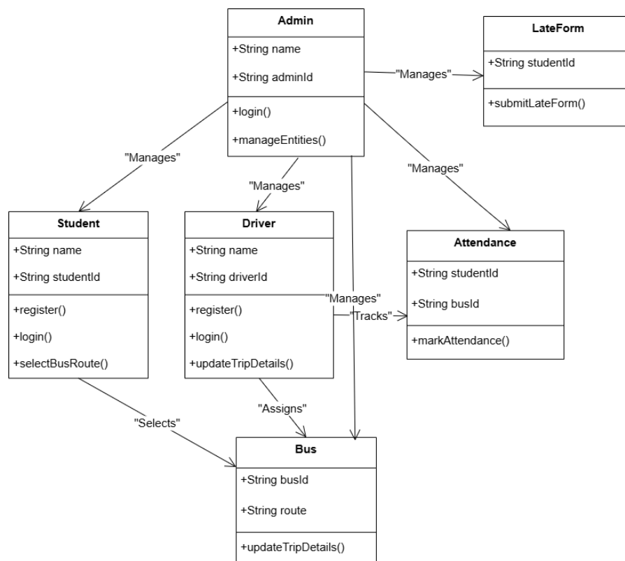
Fig.7.Class Diagram
